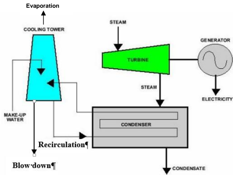
TYPICAL CLOSED-CYCLE COOLING SYSTEM
