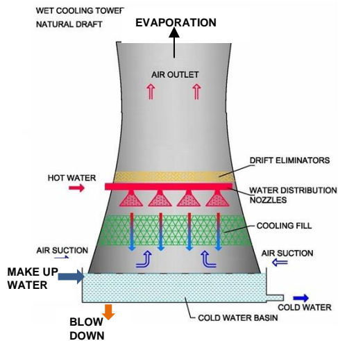
TYPICAL CLOSED-CYCLE COOLING SYSTEM
